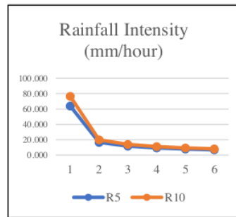
Figure 5 rainfall intensity
