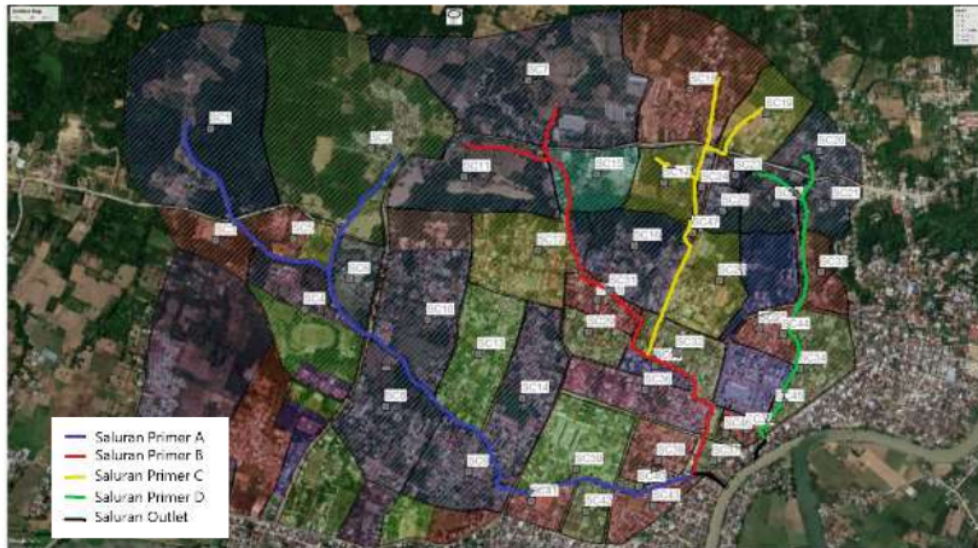
Figure 3 sub-catchment Map
