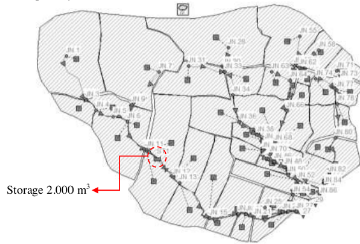
Figure 10 Storage Site Plan
