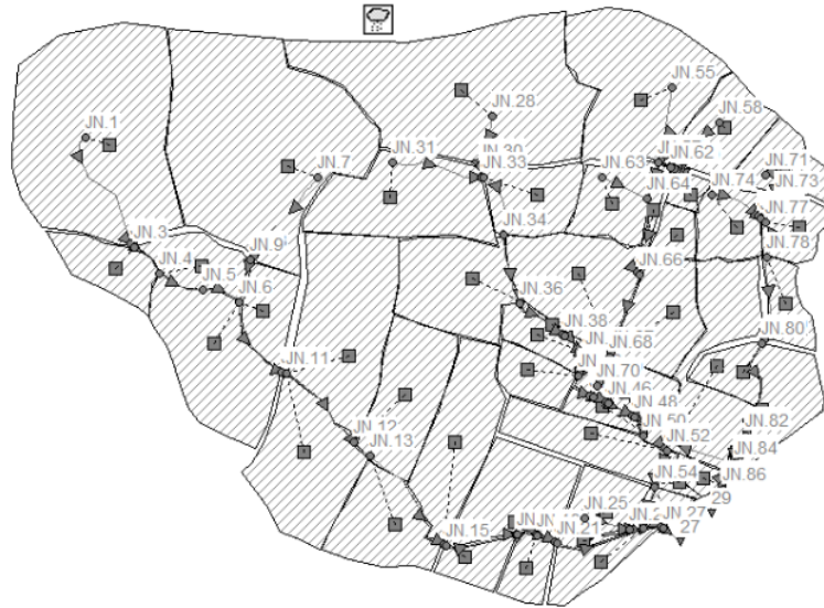
Figure 4 SWMM Modelling Map Mononobe rainfall intensity for Sengkang city
