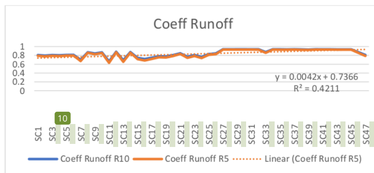
Figure 9 Coeff Runoff
